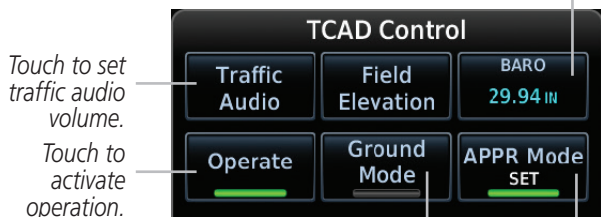
TCAD Control Menu
