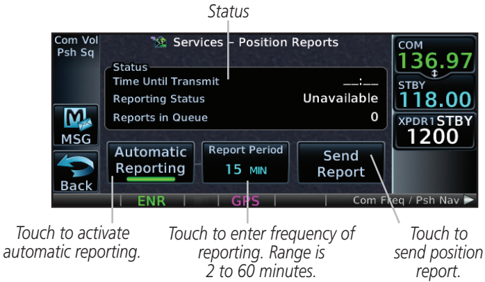
Position Reports Page
