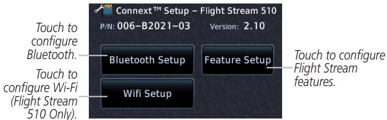
Connex Setup for Flight Stream 510
