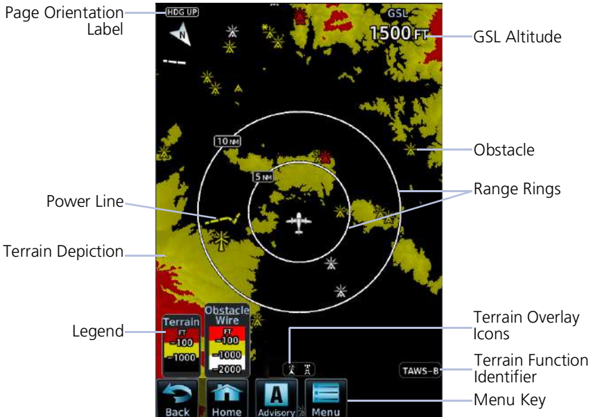
Terrain Page
