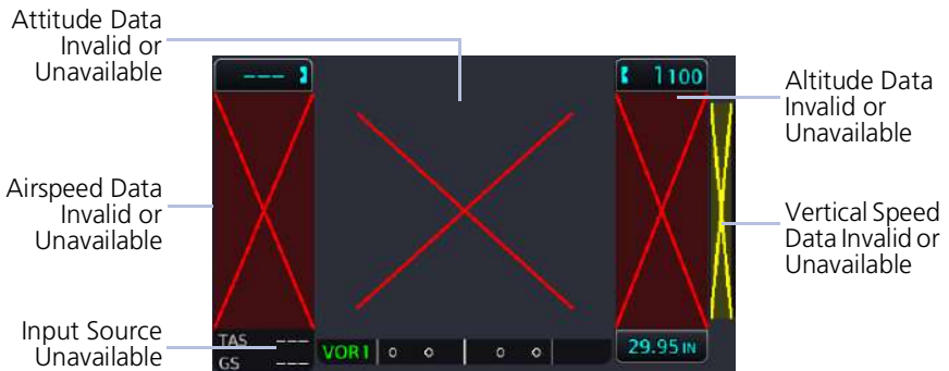
PFD
