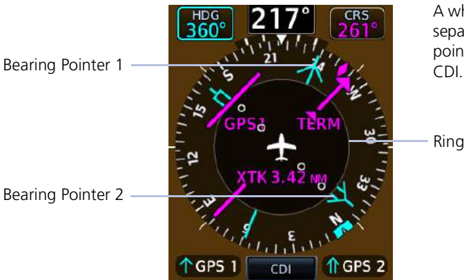
GDU 1060/700P
